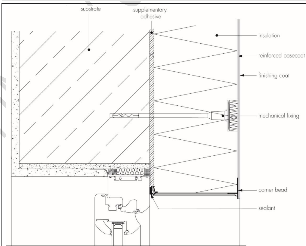
Figure 7 Window head detail
